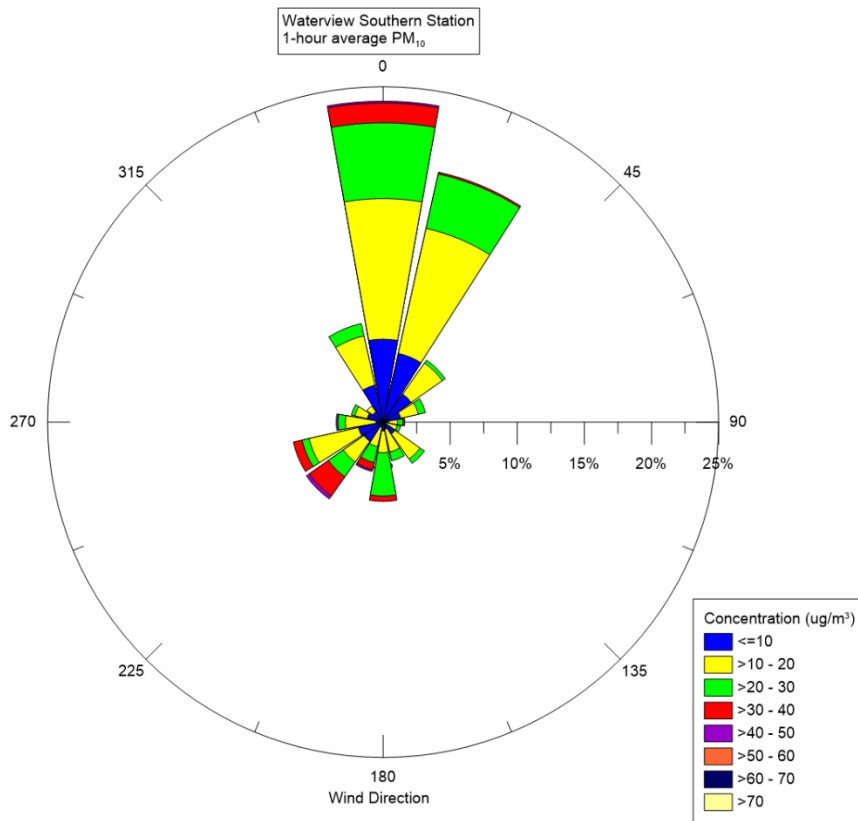
Figure D 7: Southern station 1-hour average PM 10
