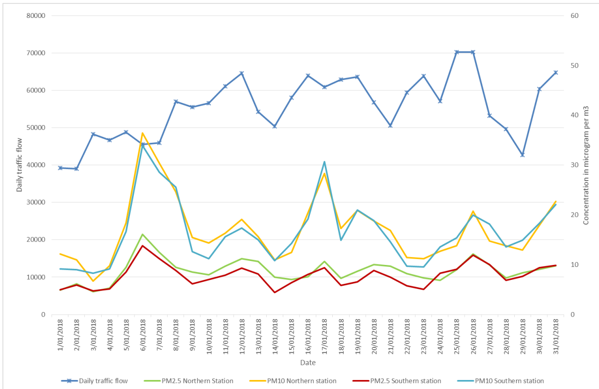
Figure 2: Waterview tunnel traffic flows and PM 2.5 /PM 10 January 2018
