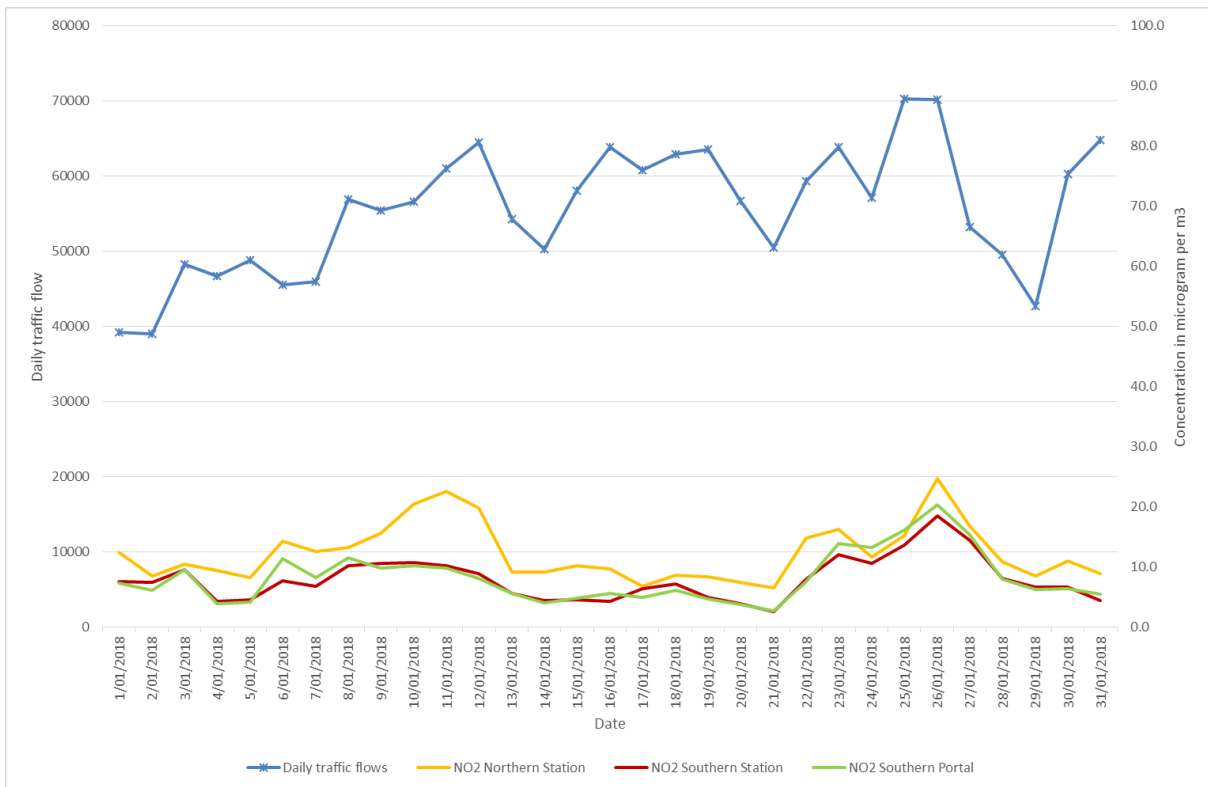
Figure 1: Waterview tunnel traffic flows and NO 2 January 2018
