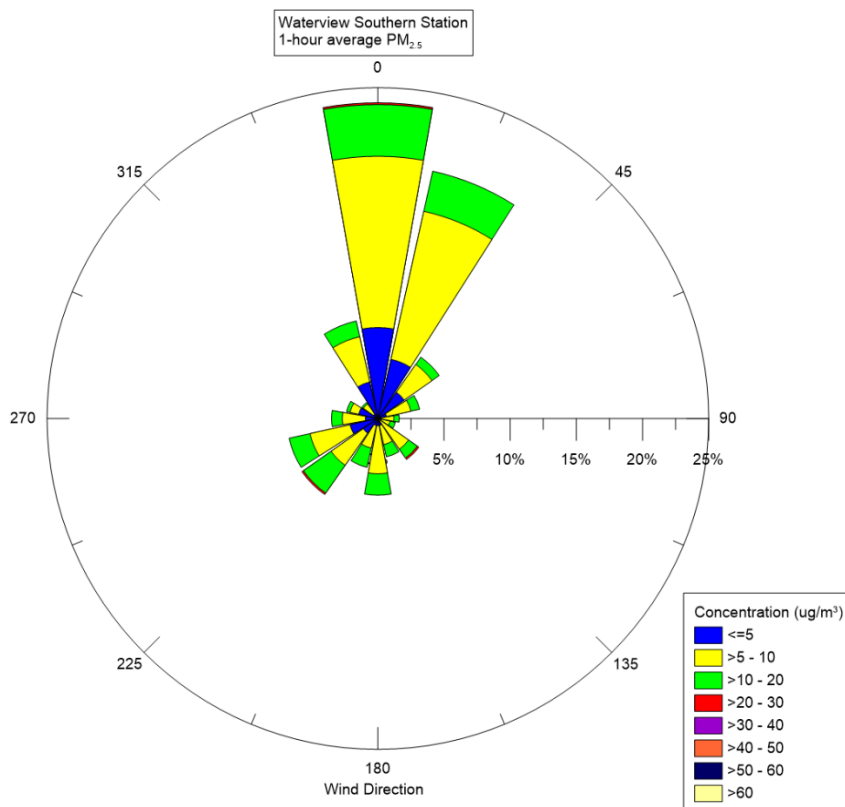
Figure D 6: Southern station 1-hour average PM 2.5
