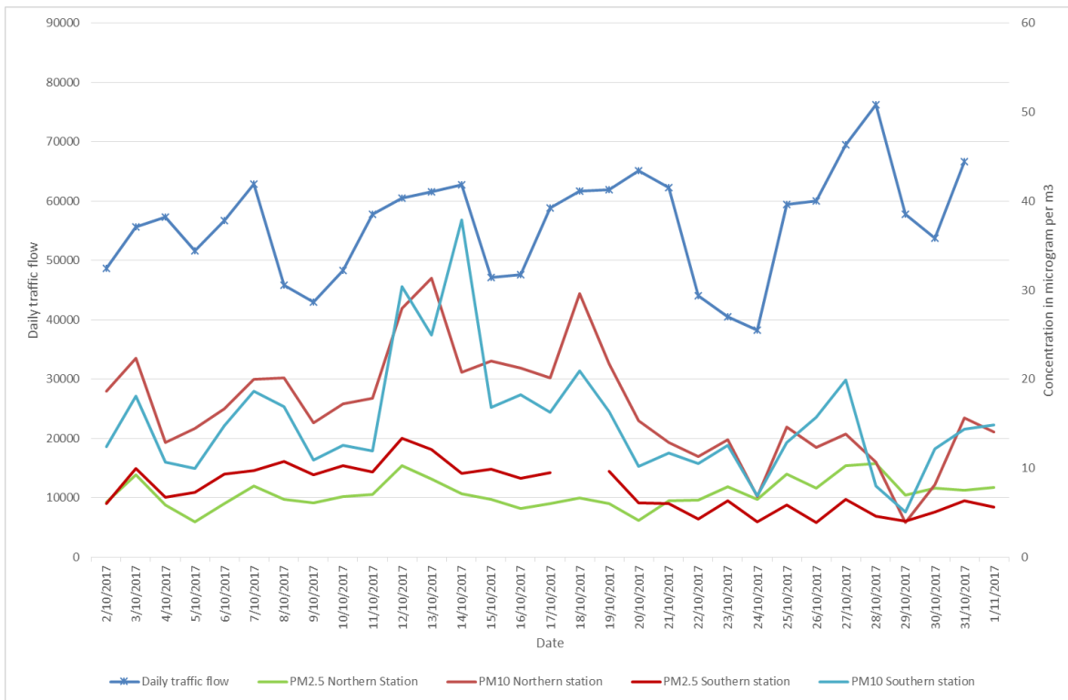
Figure 2: Waterview tunnel traffic flows and PM 2.5 /PM 10 October 2017
