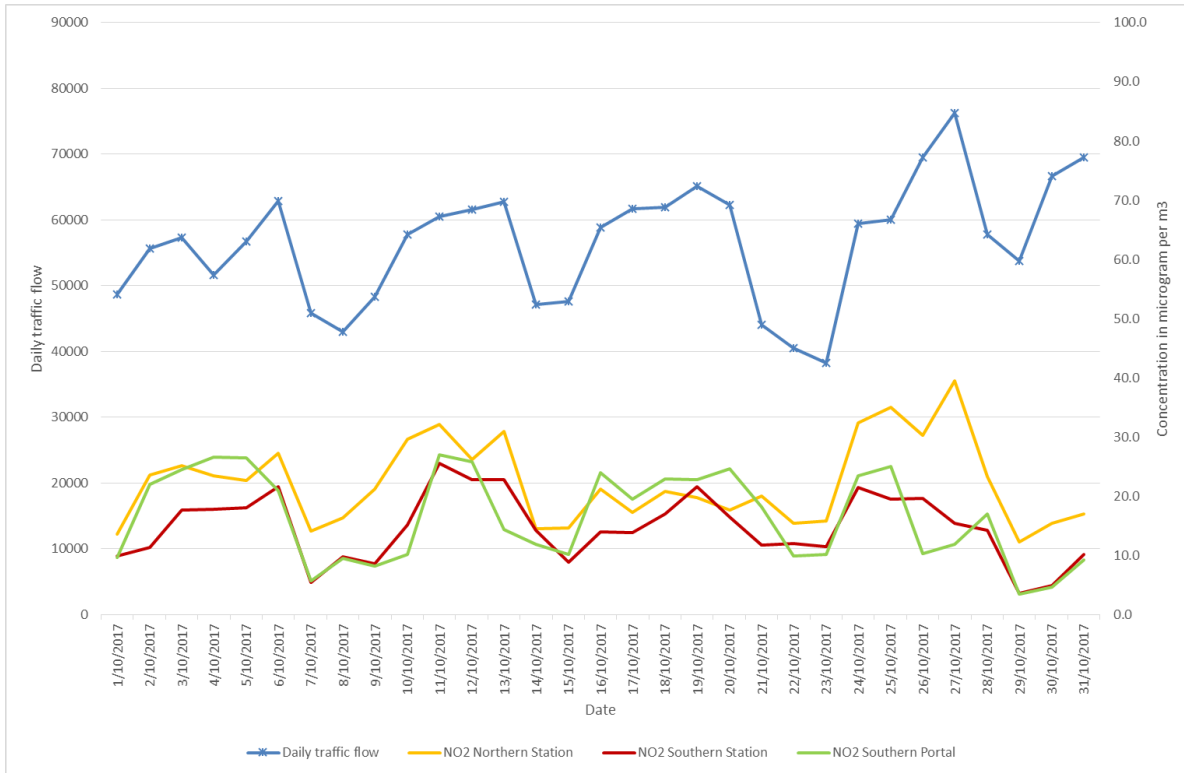
Figure 1: Waterview tunnel traffic flows and NO 2 October 2017
