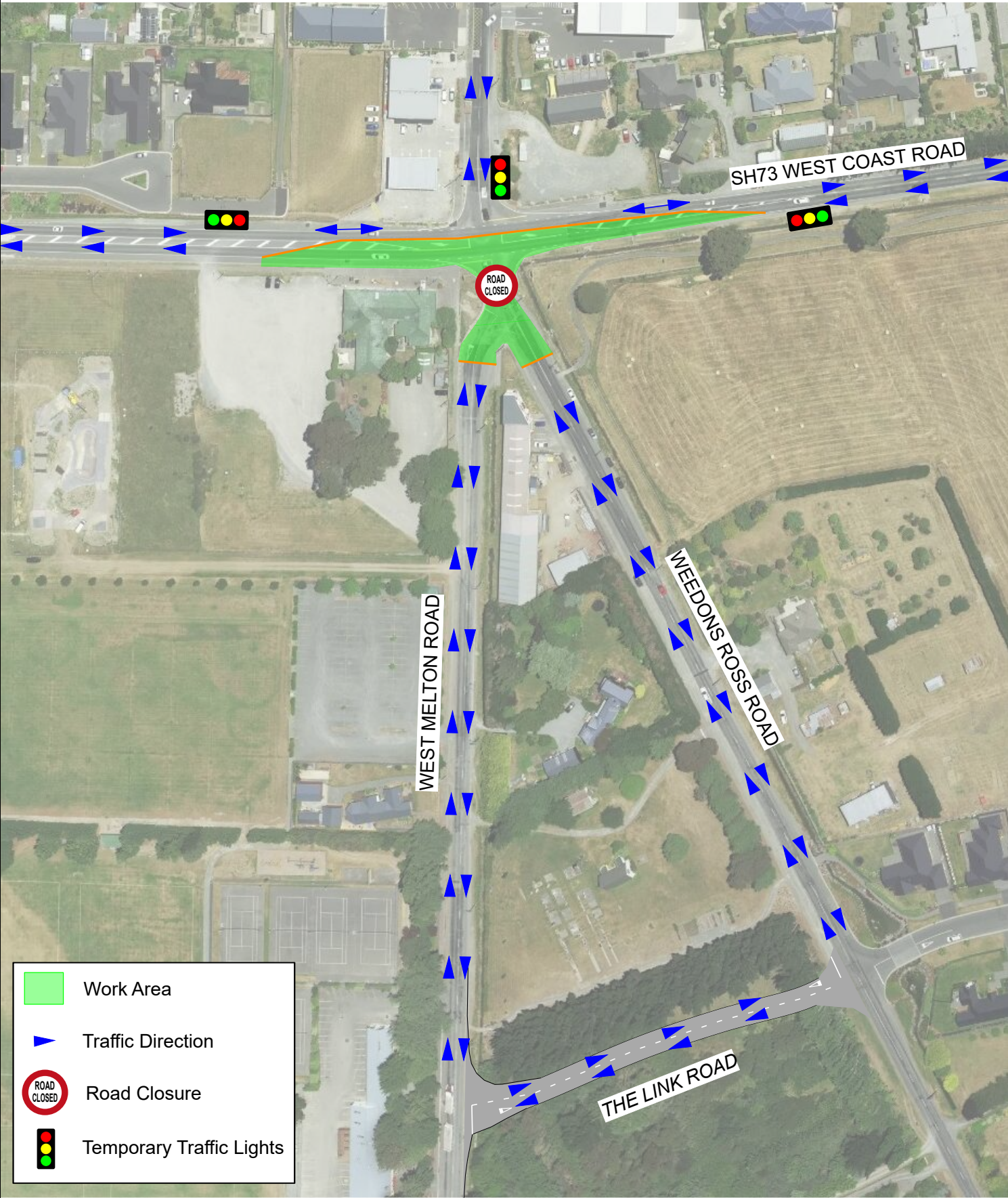
Temporary traffic management plan: closure of Weedons Ross Road (south) /SH73 West Coast Road intersection (from 9 January 2023 for a week)
