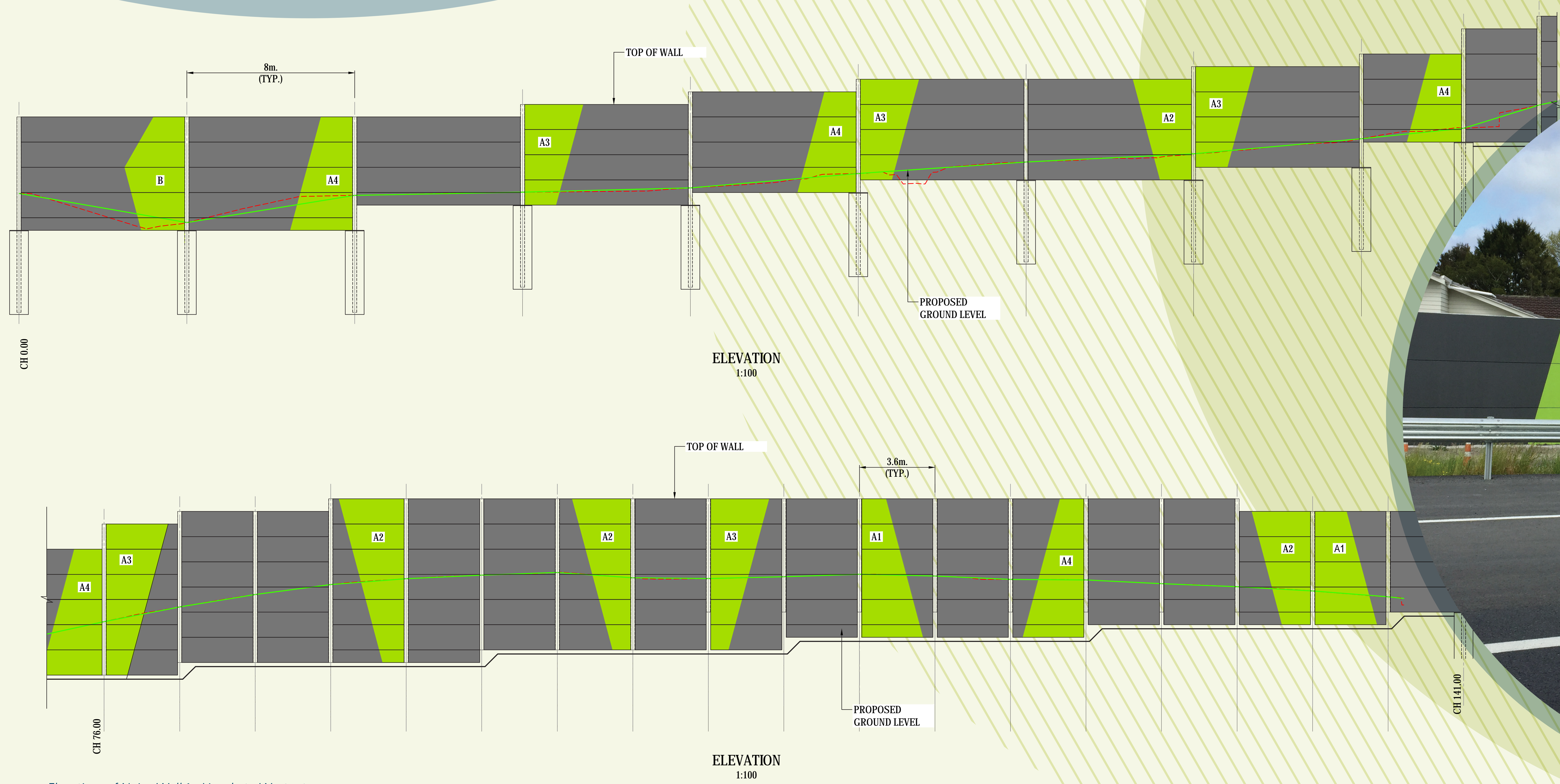
Elevations of Noise Wall 1 - Lincoln to Westgate
