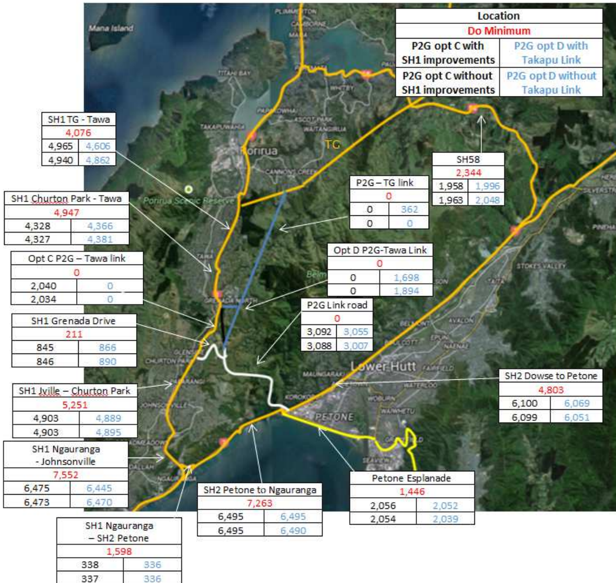
Figure 7 2031 AM Peak Hourly Traffic Flows
