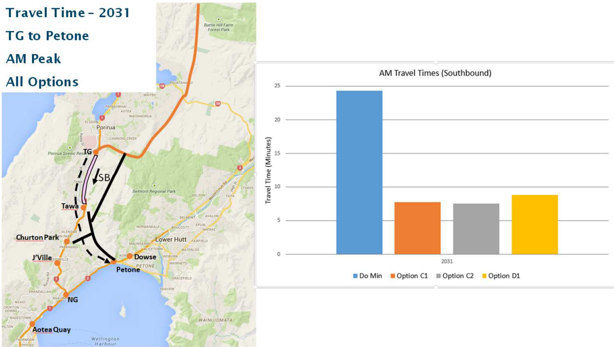
Figure 23 - Travel Time between Transmission Gully Interchange and Petone Overhead Bridge
