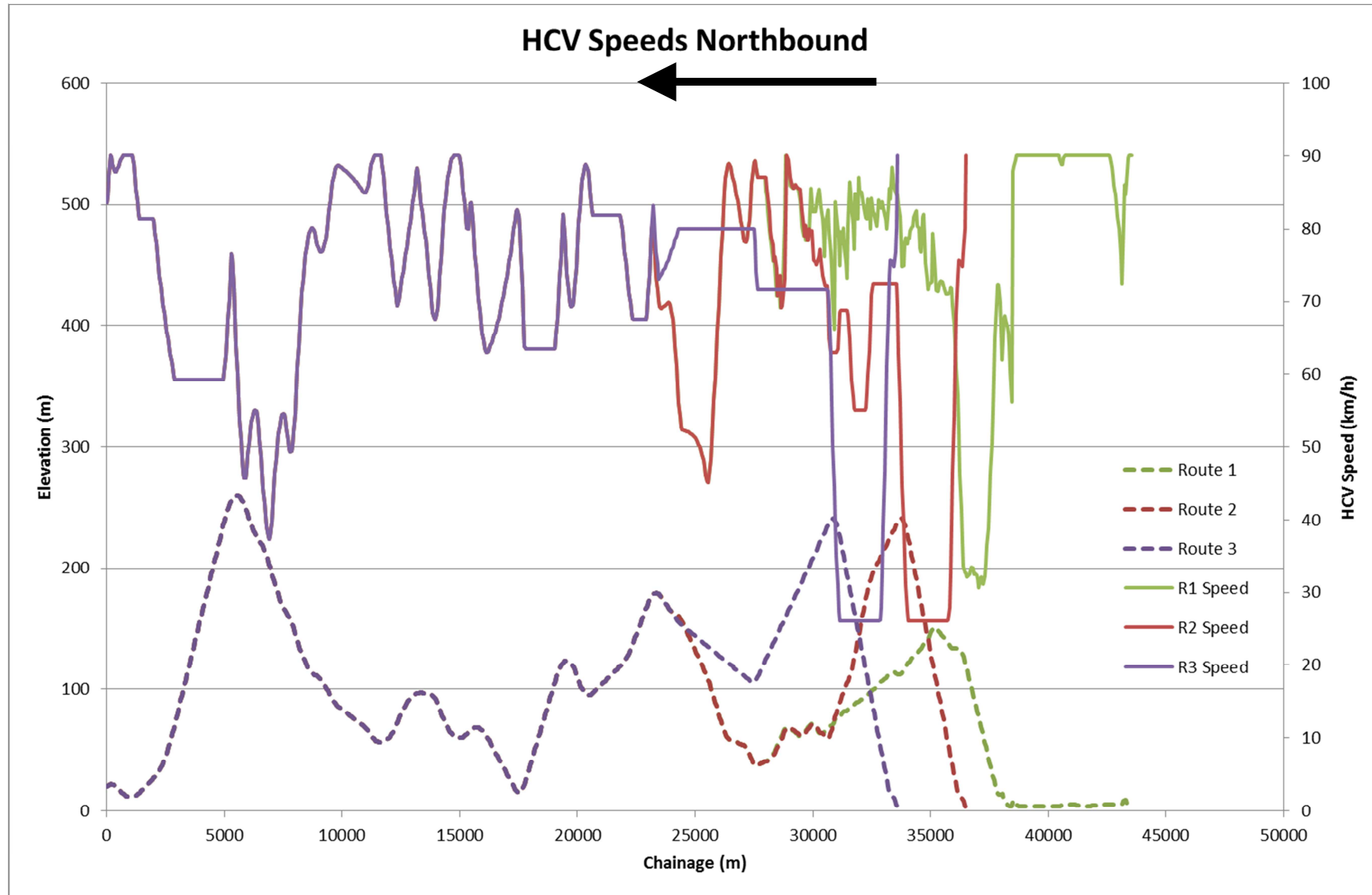
Figure 36 - Northbound Distance vs Speed
