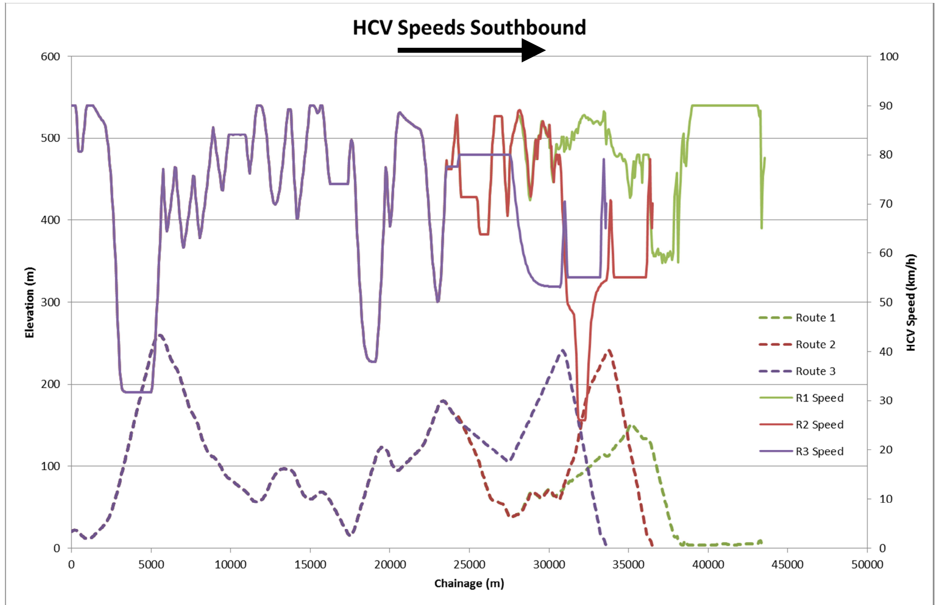
Figure 35 - Southbound Distance vs Speed
