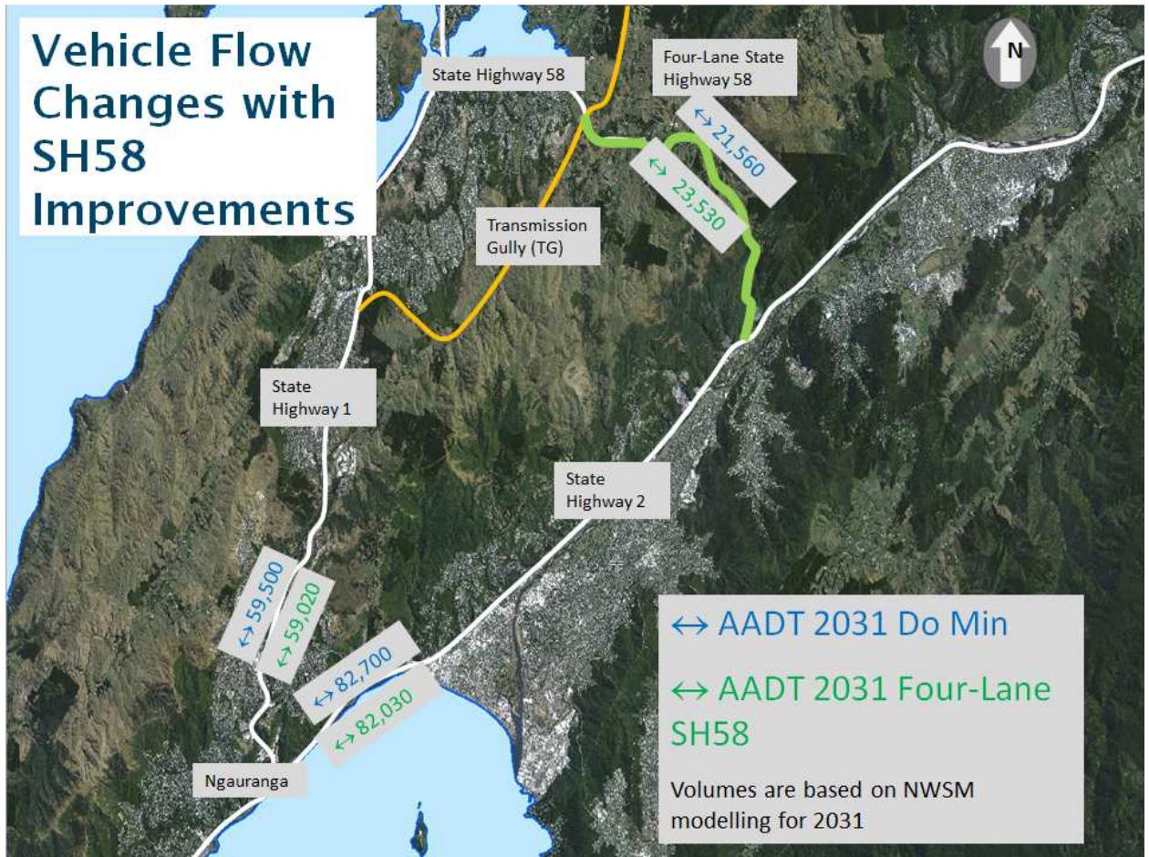
Figure 37 - Impact of SH58 Four Lining on Annual Average Daily Traffic (AADT) Flows in 2031
