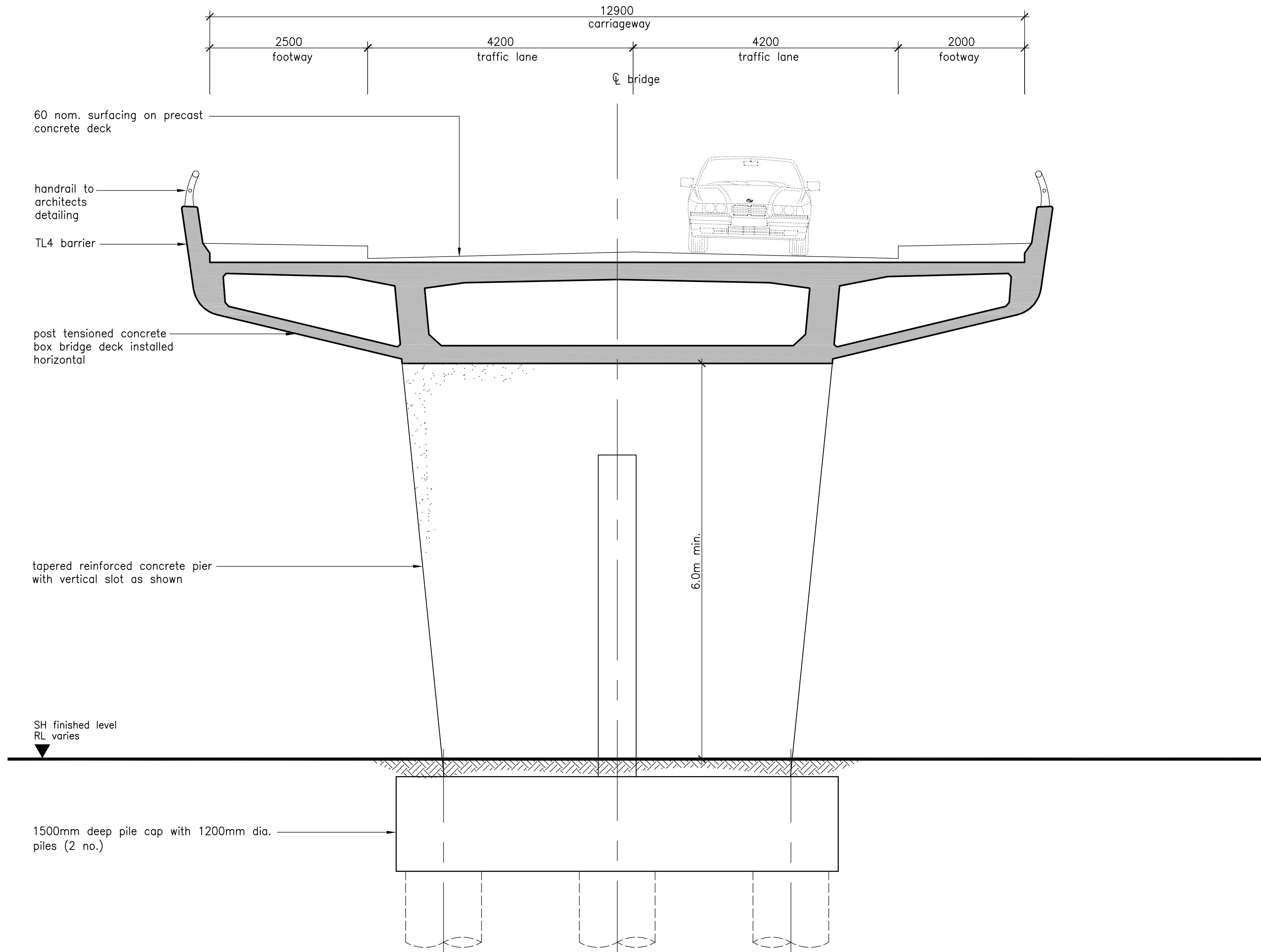
1 S06 1:50 bridge cross section at pier
