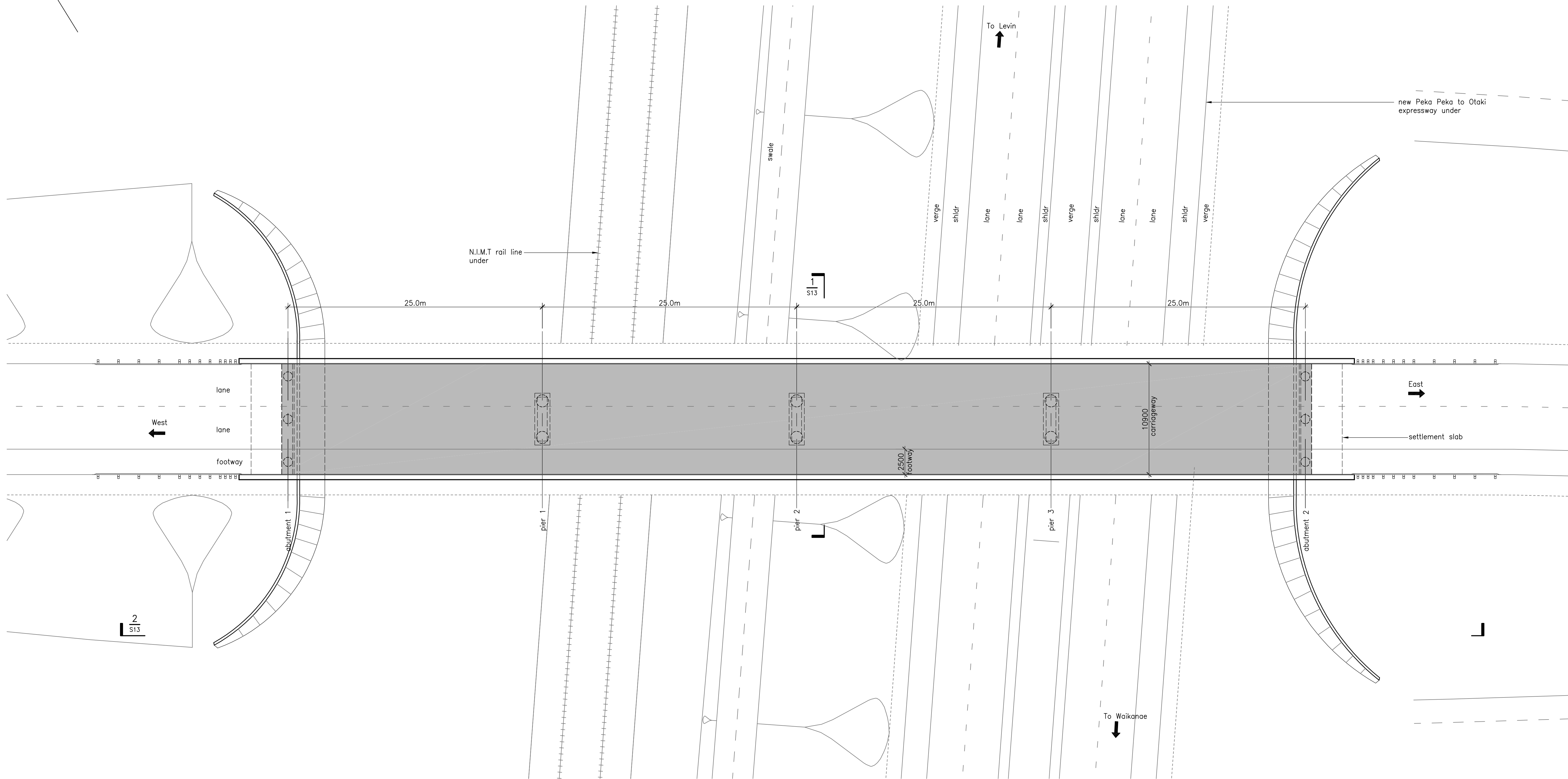
bridge general arrangement plan
