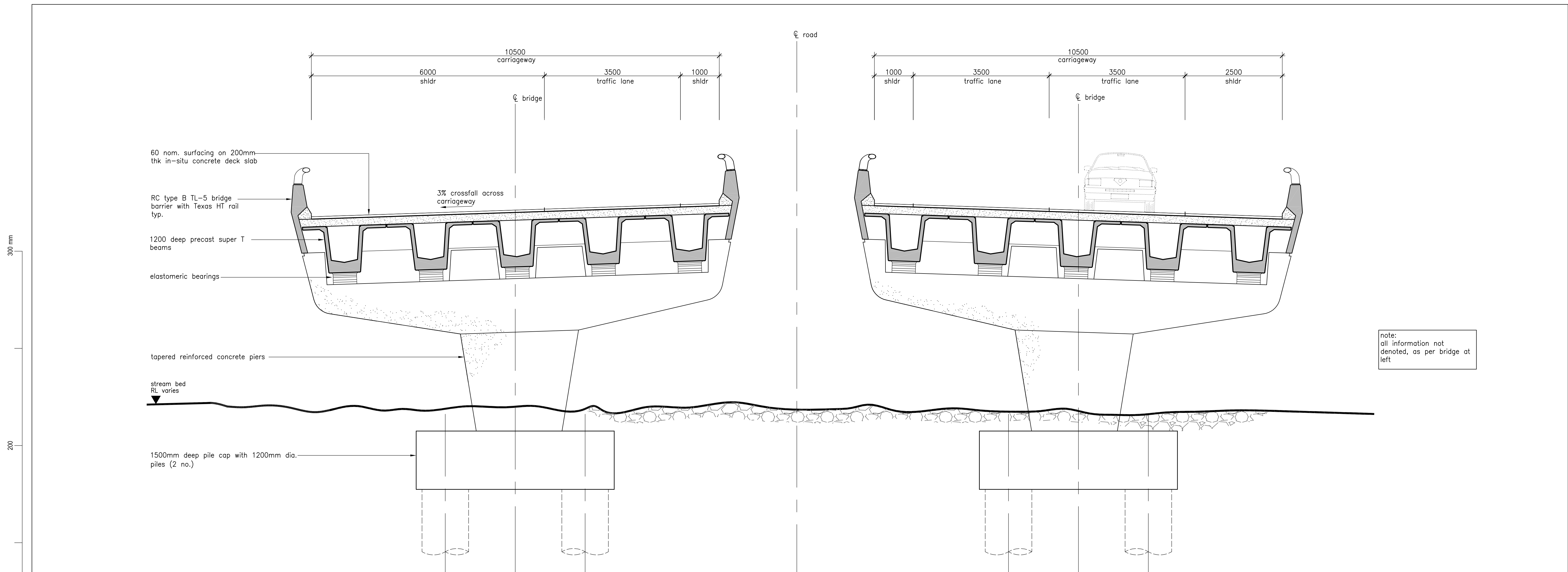
1 S02 bridge cross section at pier 1:50
