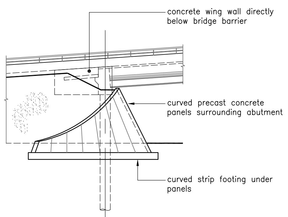
3 1:200 bridge part elevation showing precast abutment surround
