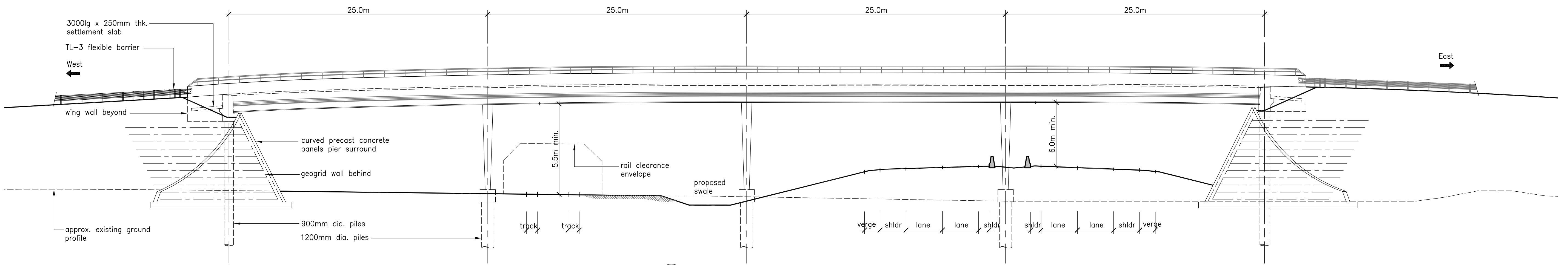
2 S12 1:200 bridge elevation
