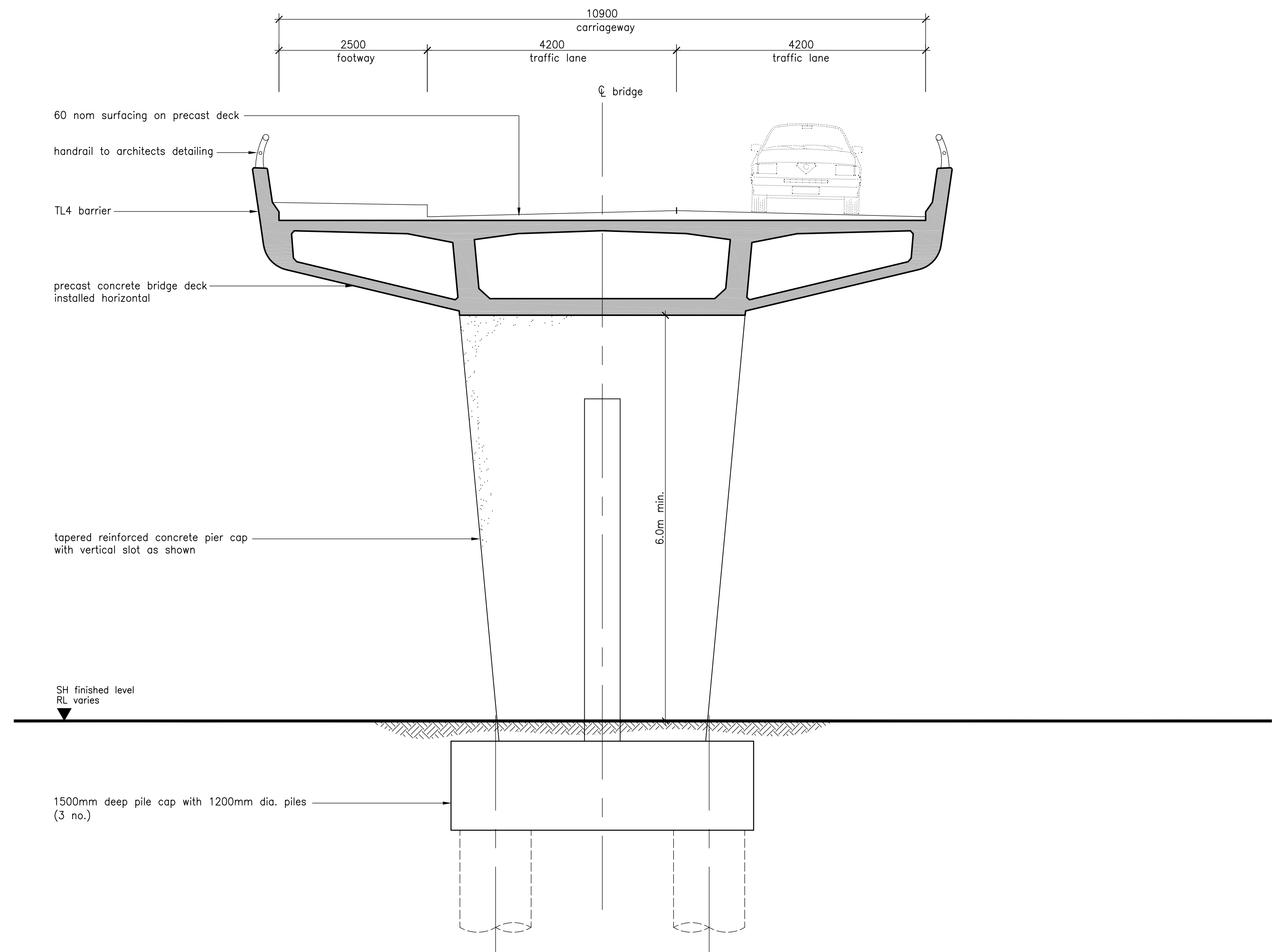
1 S12 1:50 bridge cross section at pier
