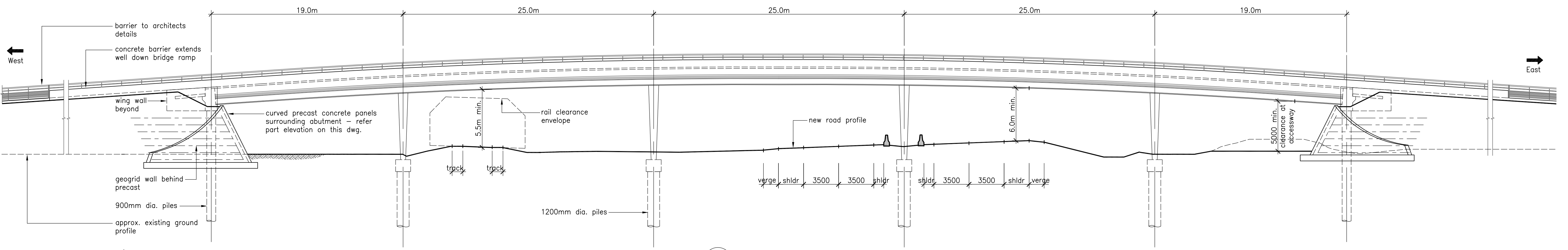
2 S06 1:200 bridge elevation
