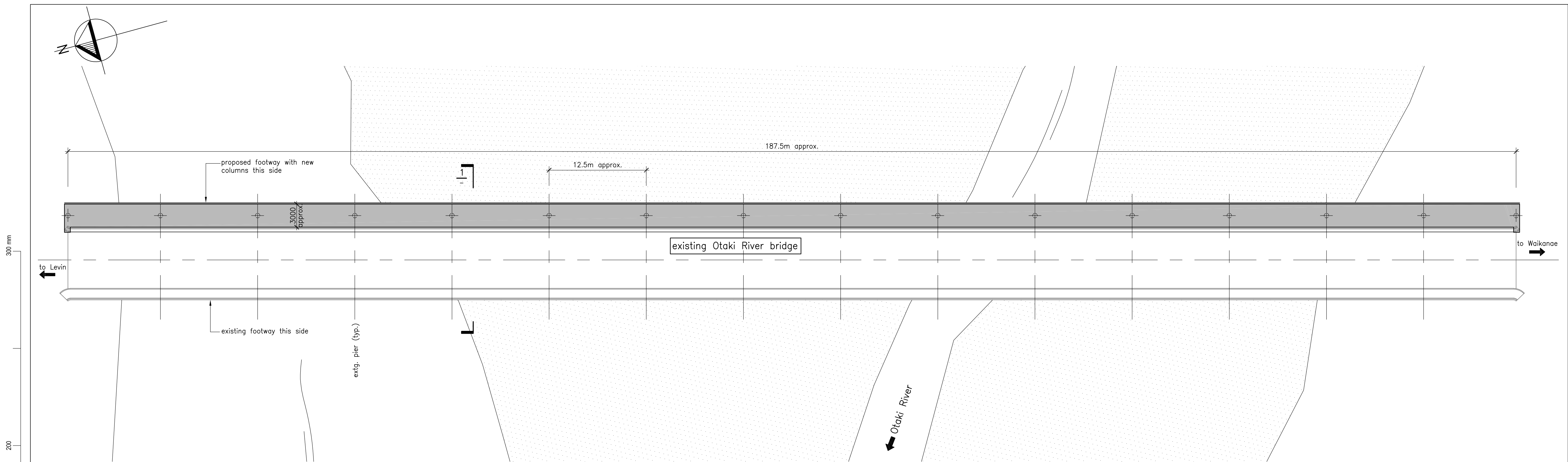
bridge general arrangement plan 1:250
