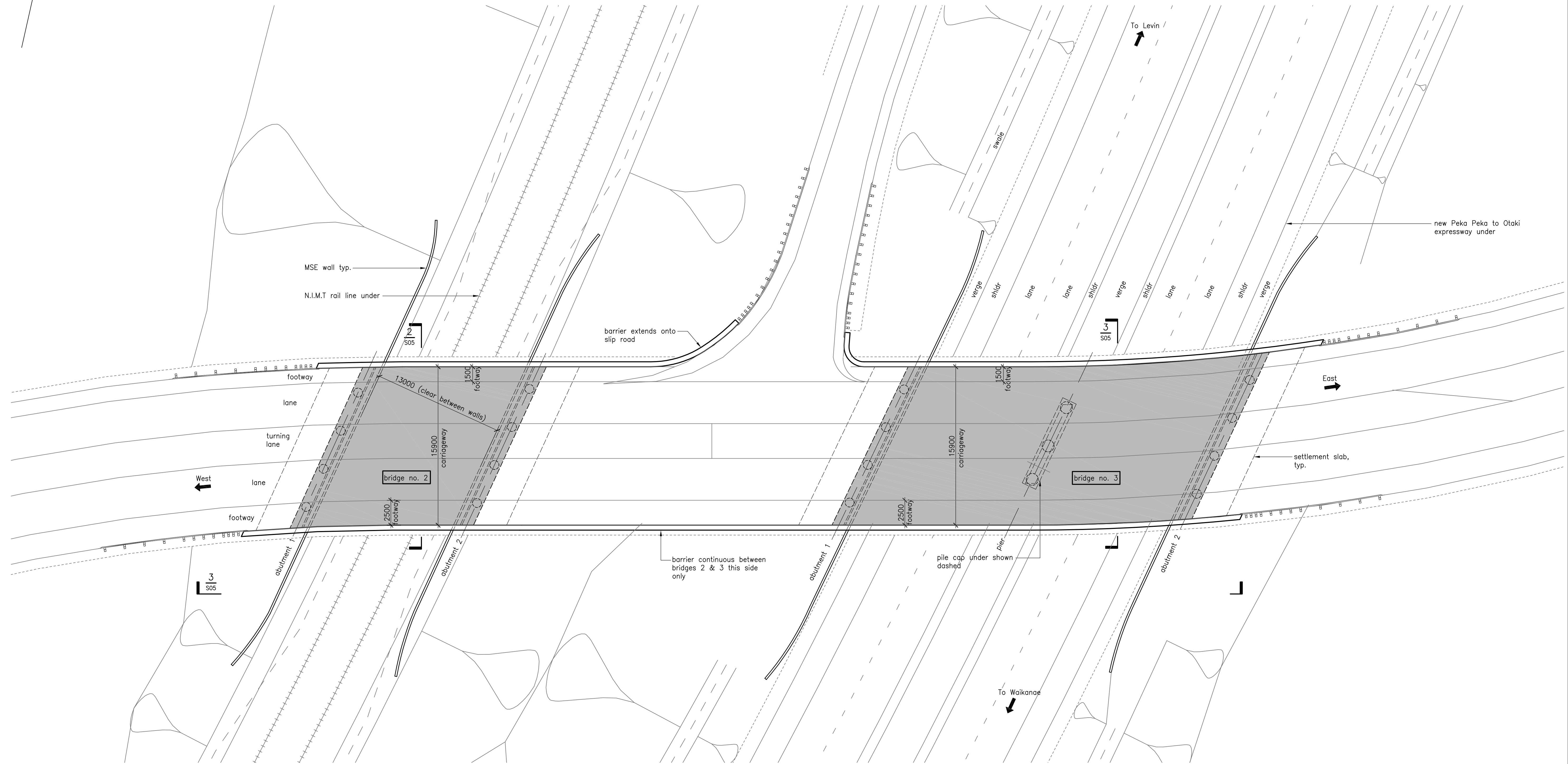
bridges general arrangement plan
