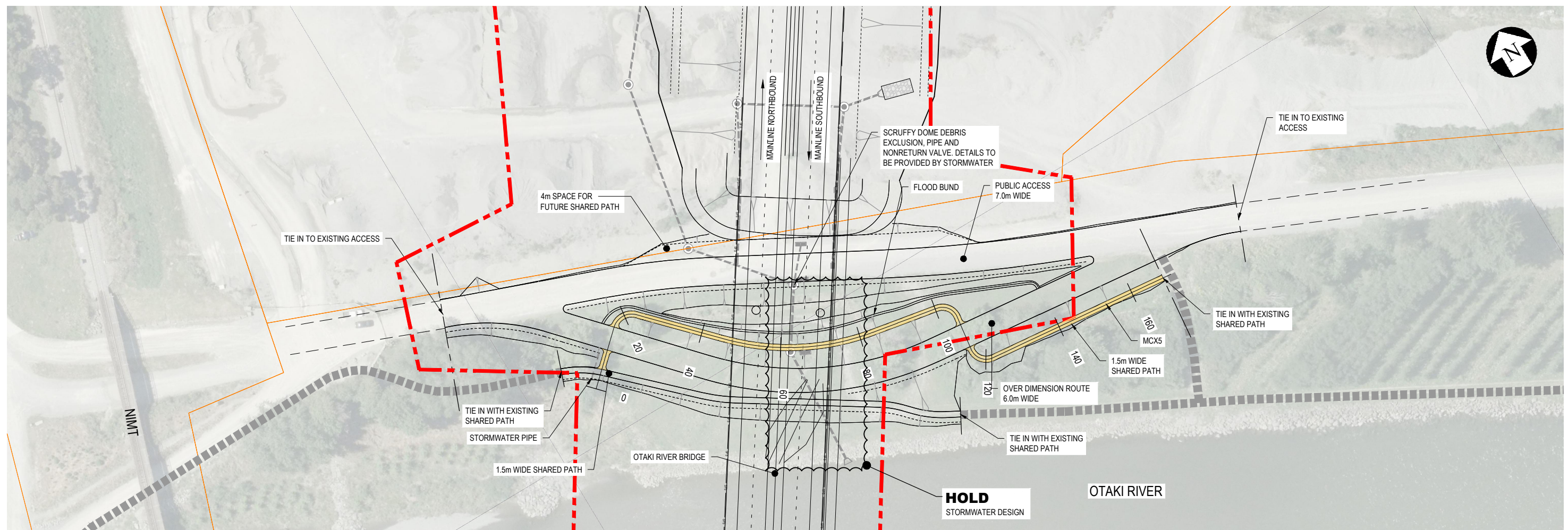
PLAN SHARED PATH - ALTERNATIVE ROUTE SCALE 1:500 (A1)
