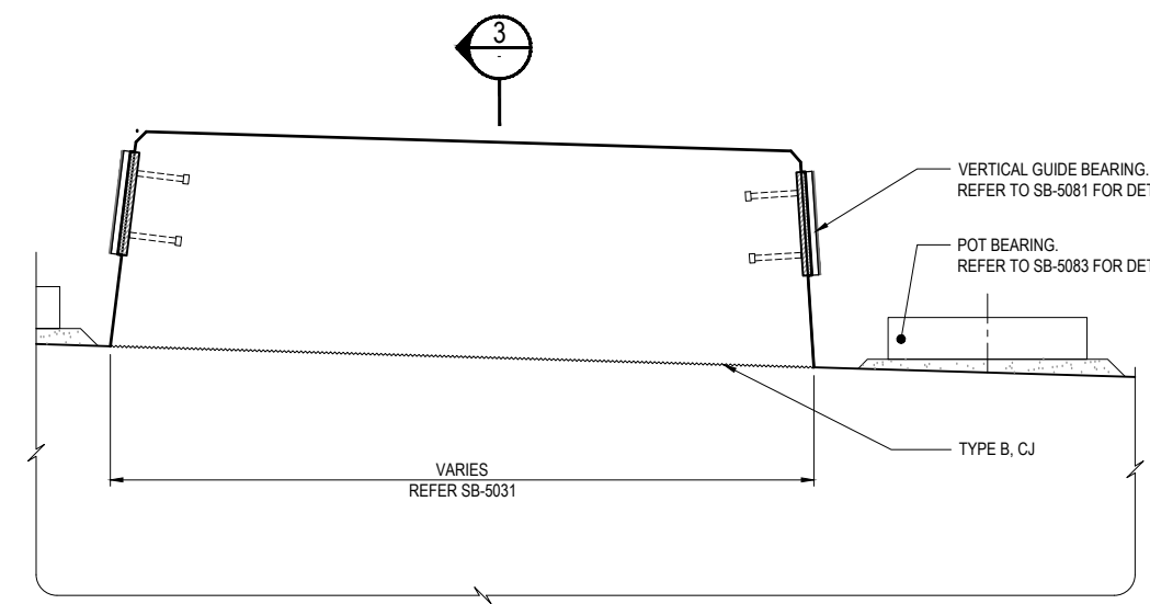
A DETAIL - SHEAR KEY SB-5031 SCALE 1:10
