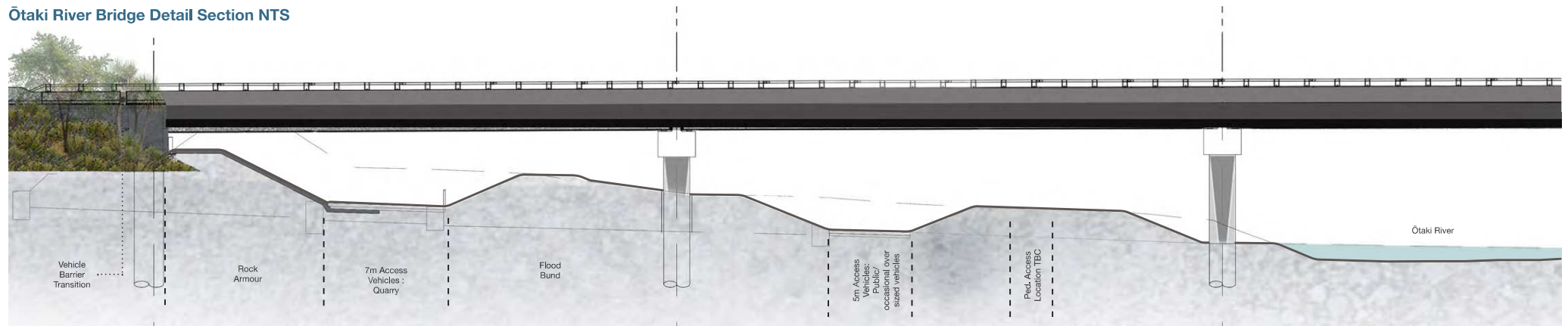
Figure 87. Ōtaki River Bridge Sections
