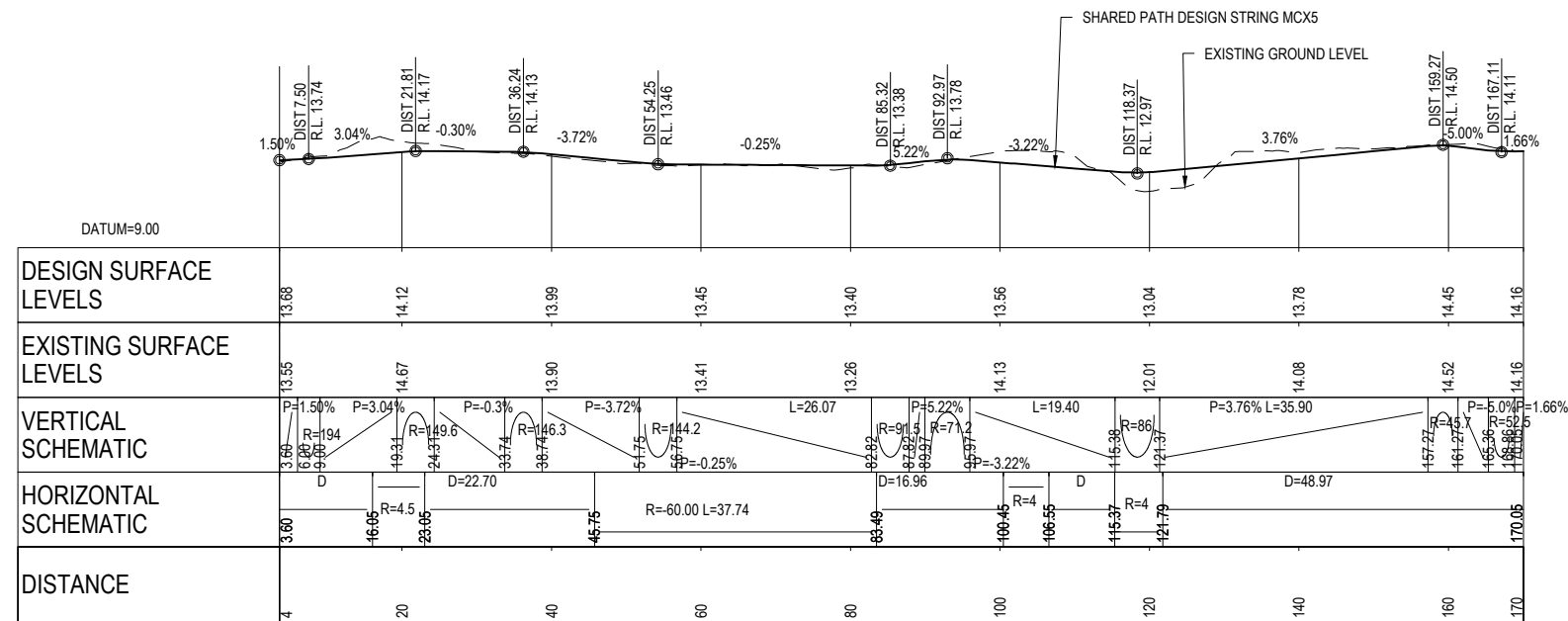
LONGITUDINAL SECTION ON CONTROL STRING MCX5 SCALE HORIZ=1:500 VERT=1:200
