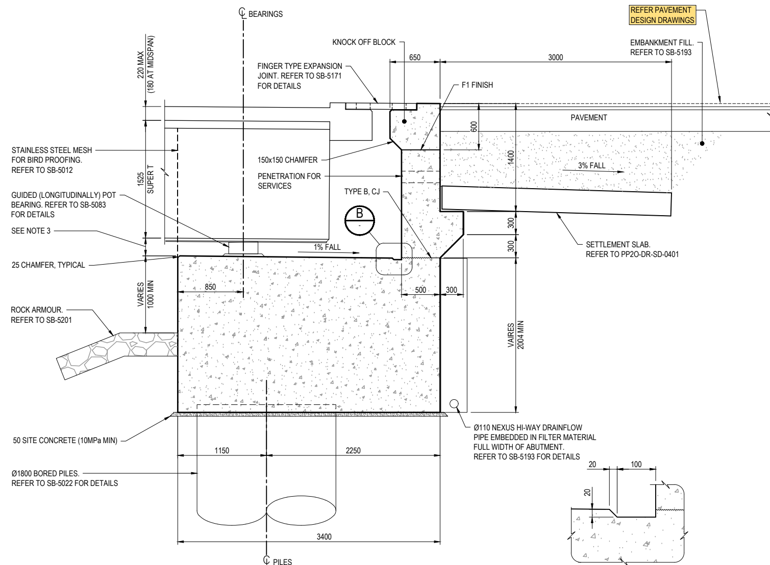
1 SECTION SB-5031 SCALE 1:25
