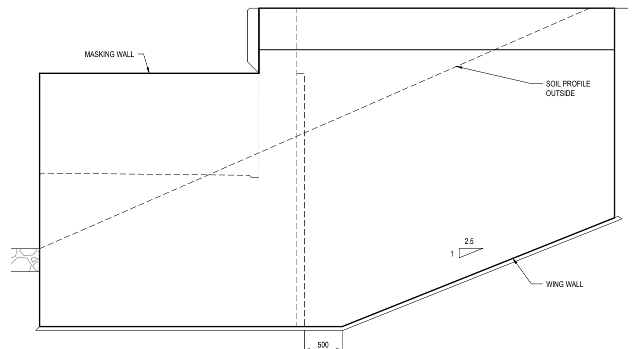
3 SECTION SB-5031 SCALE 1:25
