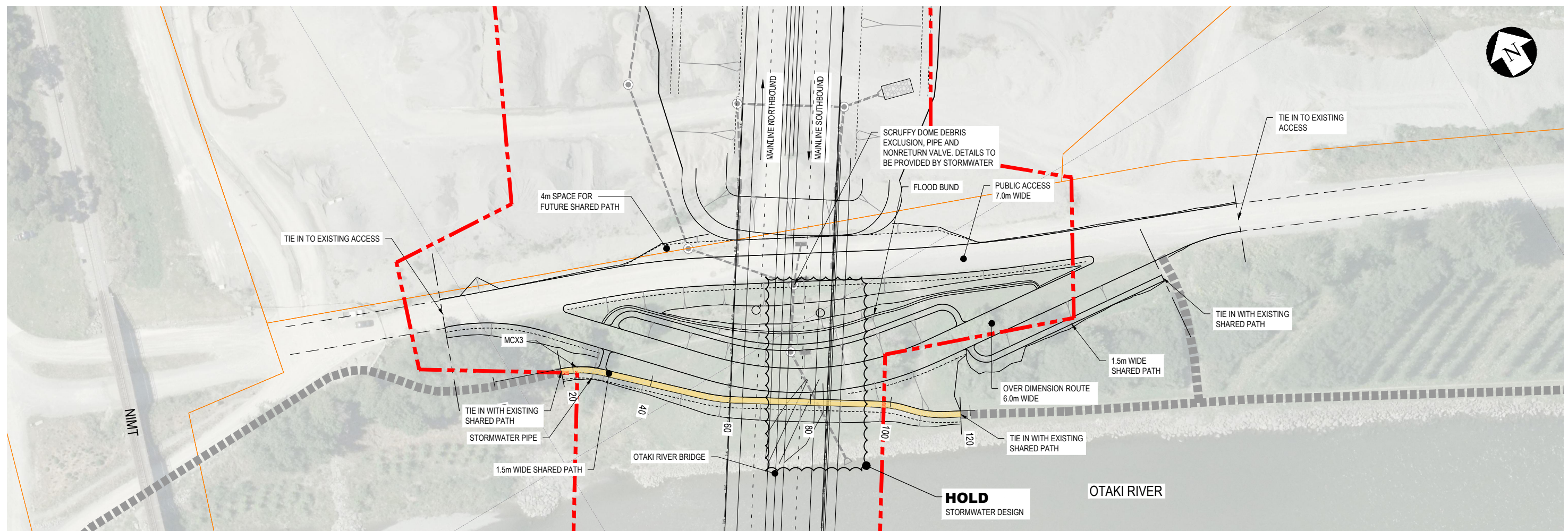
PLAN - SHARED PATH SCALE 1:500 (A1)
