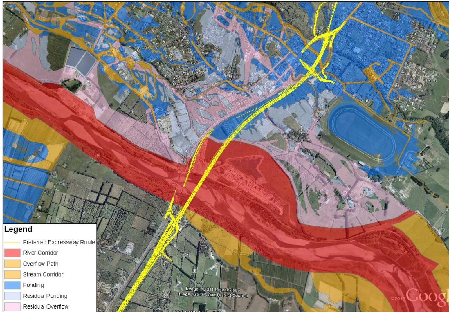
Figure D-1 Composite GWRC / KCDC flood hazard map for existing situation on Ōtaki River and floodplain
