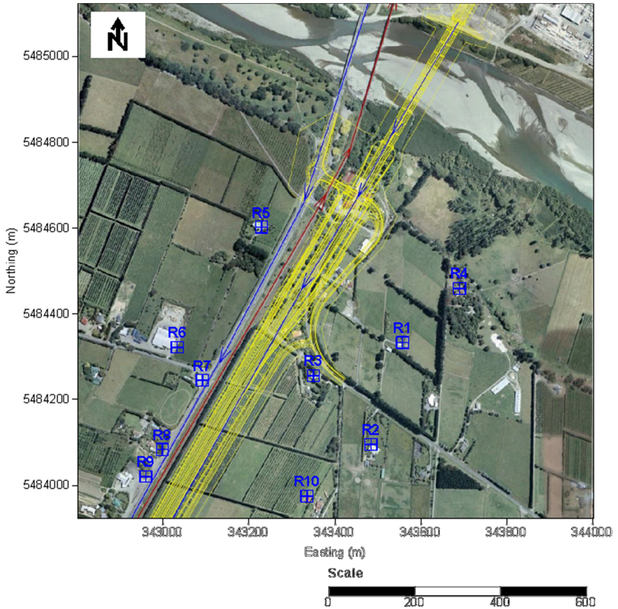
Figure C-2 Traffic Links Modelled for South Otaki, 'With Project' 2021
