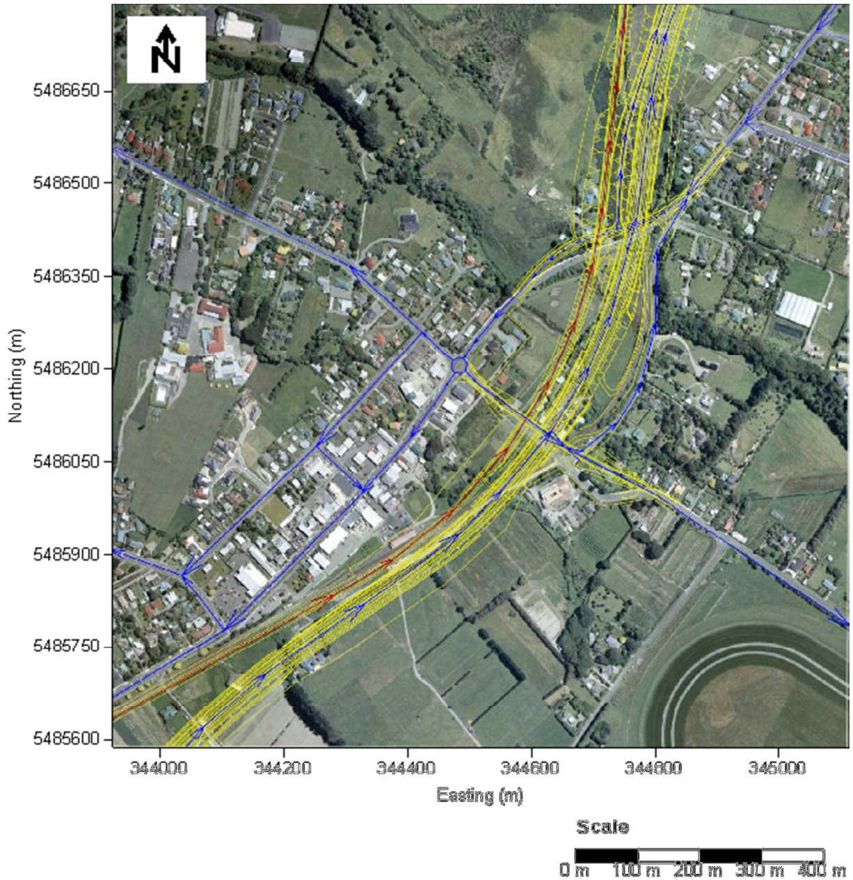
Figure C-1 Traffic Links Modelled for Otaki, 'With Project' 2021
