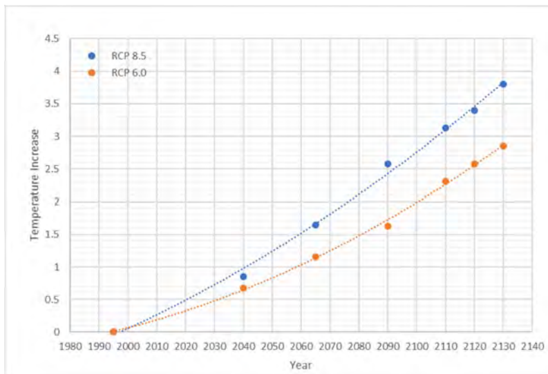
Figure 4-10: Estimated temperature increase to 2130
