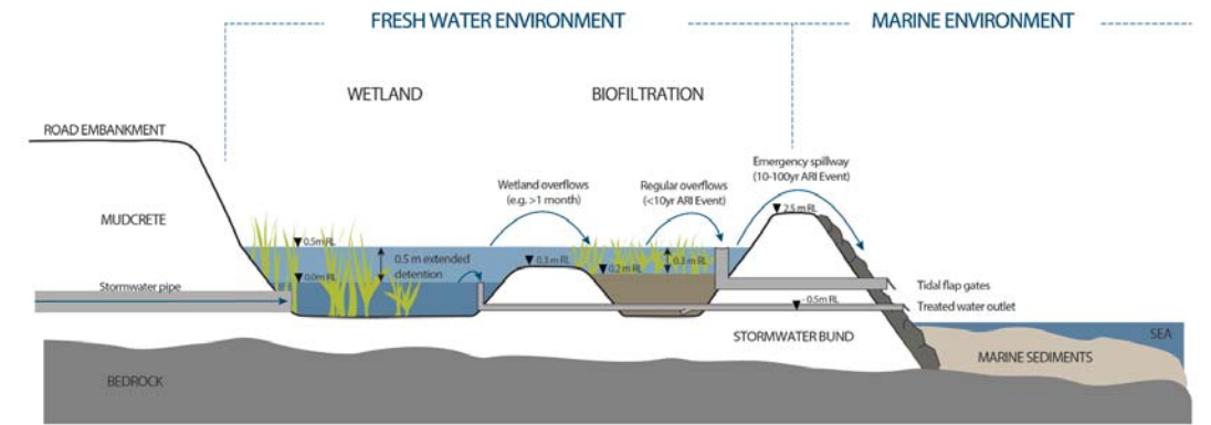
Stormwater treatment process (details to be confirmed during detailed design)
