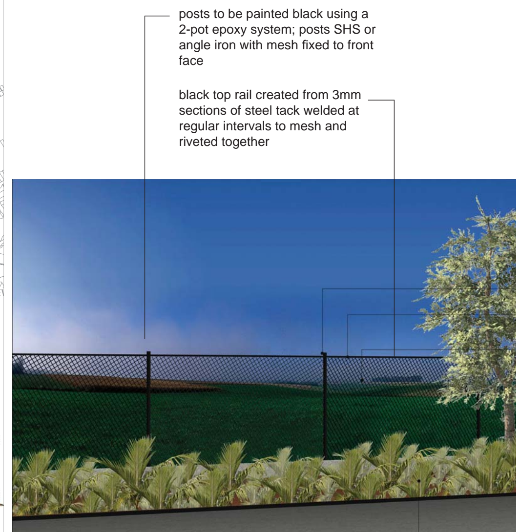
Figure B-28: Proposed fence concept – SH20
