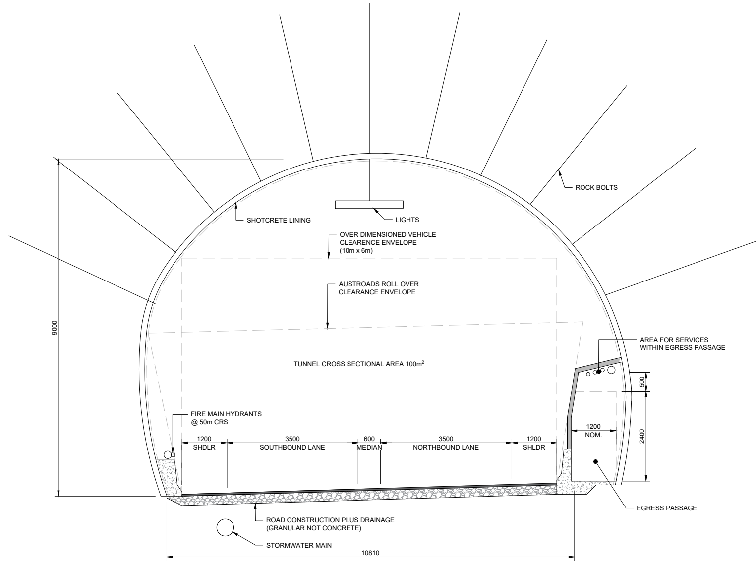
TYPICAL MID SECTION TUNNEL CROSS SECTION SCALE: 1:50
