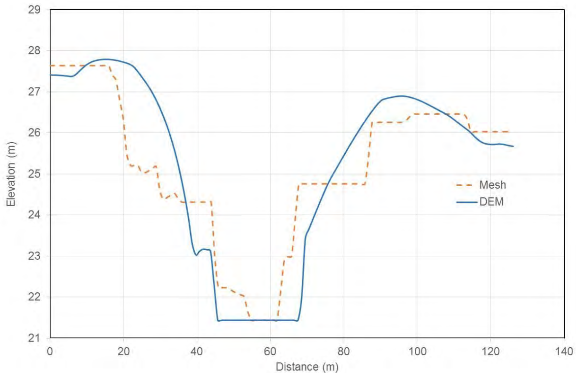
Figure 53 – Comparison of cross-sections of the Hōteō River extracted from LIDAR based DEM and the model mesh
