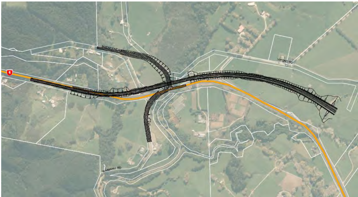
Figure 7-8: New offline bridge and grade separated intersection (JG02)
