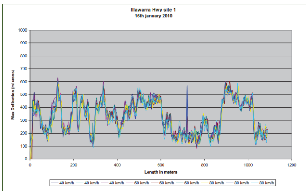
Figure 2.4-1: Vehicle Speed Comparison – from Queensland Trial of TSD (Weligamage et al)
