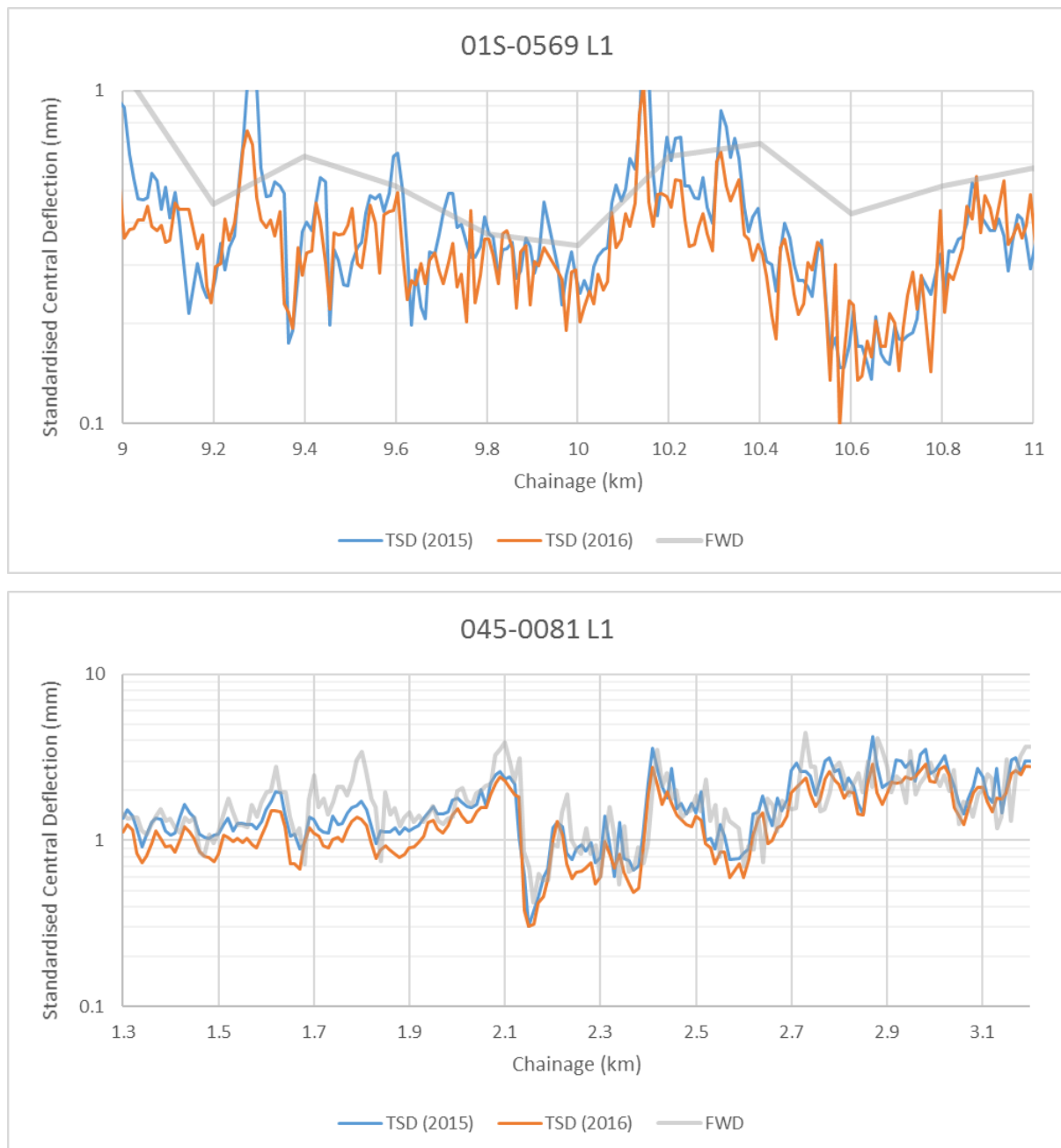
Figure 2.4-2: Two examples comparison of TSD runs (2015 - 2016) with FWD data
